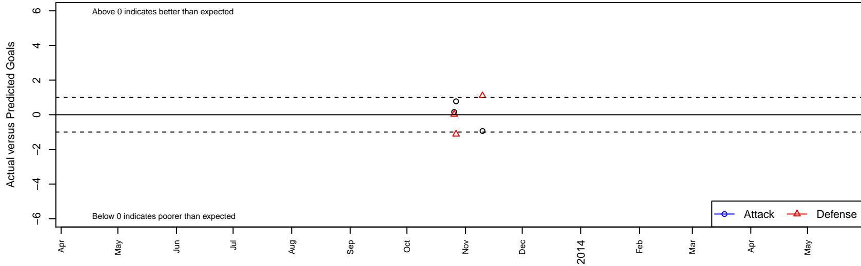
Oakland Select B98 Dots are actual minus expected GF (blue circles) and GA (red triangles). Blue line is smoothed change in attack strength. Red is smoothed change in defense strength.
